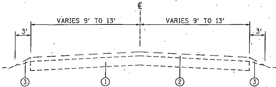
EXISTING TYPICAL SECTION LOCATION #1 - MARINE/ST.JACOB RD. NOT TO SCALE
