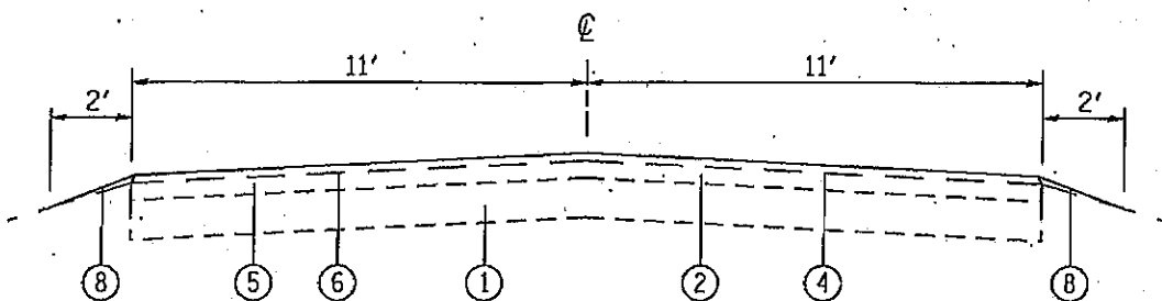
PROPOSED TYPICAL SECTION LOCATION #2 - HIGHLAND ROAD NOT TO SCALE STA 0+00 TO STA 8+76 STA 13+32 TO STA 20+60 STA 30+90 TO STA 33+70
