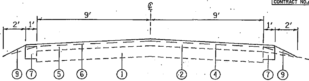
PROPOSED TYPICAL SECTION LOCATION #1 - MARINE/ST.JACOB RD. NOT TO SCALE STA 186+30 TO STA 250+47
