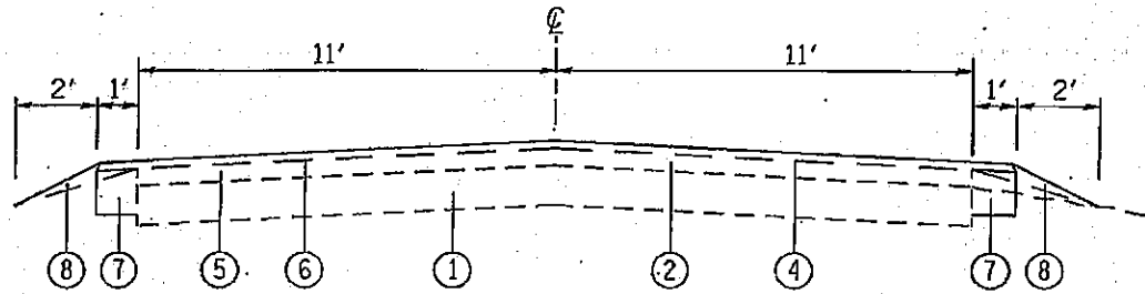
PROPOSED TYPICAL SECTION LOCATION #2 - HIGHLAND ROAD NOT TO SCALE STA 8+75 TO STA 13+32 STA 20+60 TO STA 30+90 STA 33+70 TO STA 40+30
