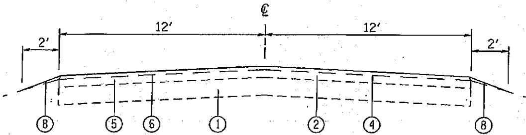
PROPOSED TYPICAL SECTION LOCATION #1 - MARINE/ST.JACOB RD. NOT TO SCALE STA 250+47 TO STA 257+50
