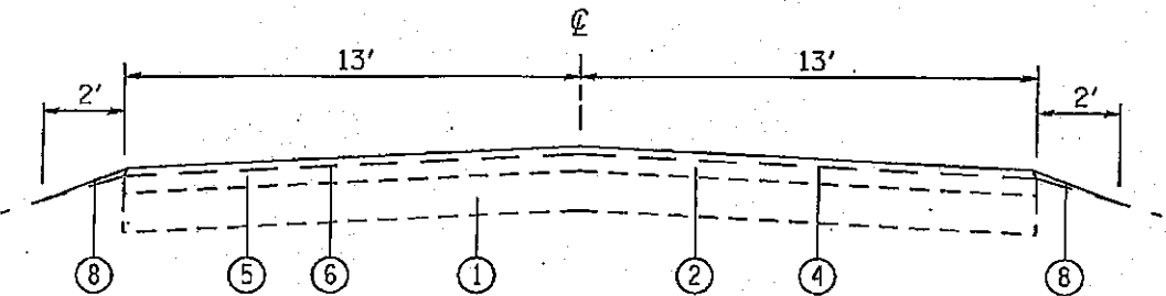
PROPOSED TYPICAL SECTION LOCATION #1 - MARINE/ST.JACOB RD. NOT TO SCALE STA 257+50 TO STA 259+90
