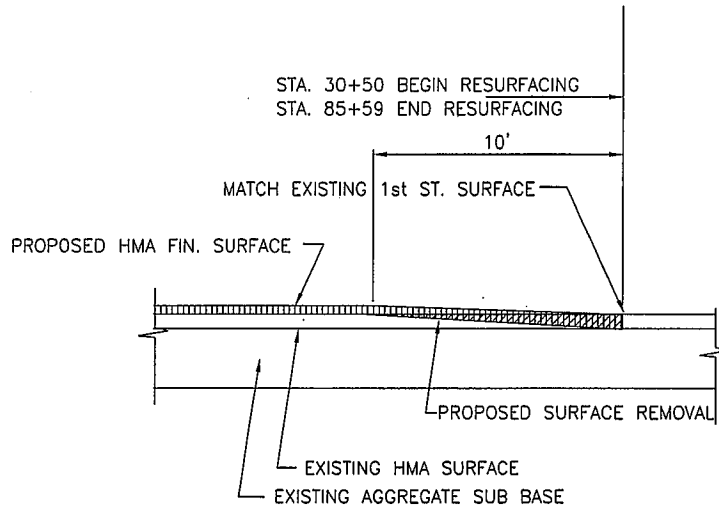
BUTT JOINT AT HEADERS
