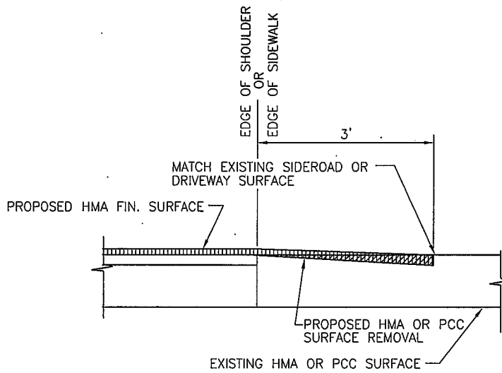
BUTT JOINT AT SIDEROADS AND DRIVES
