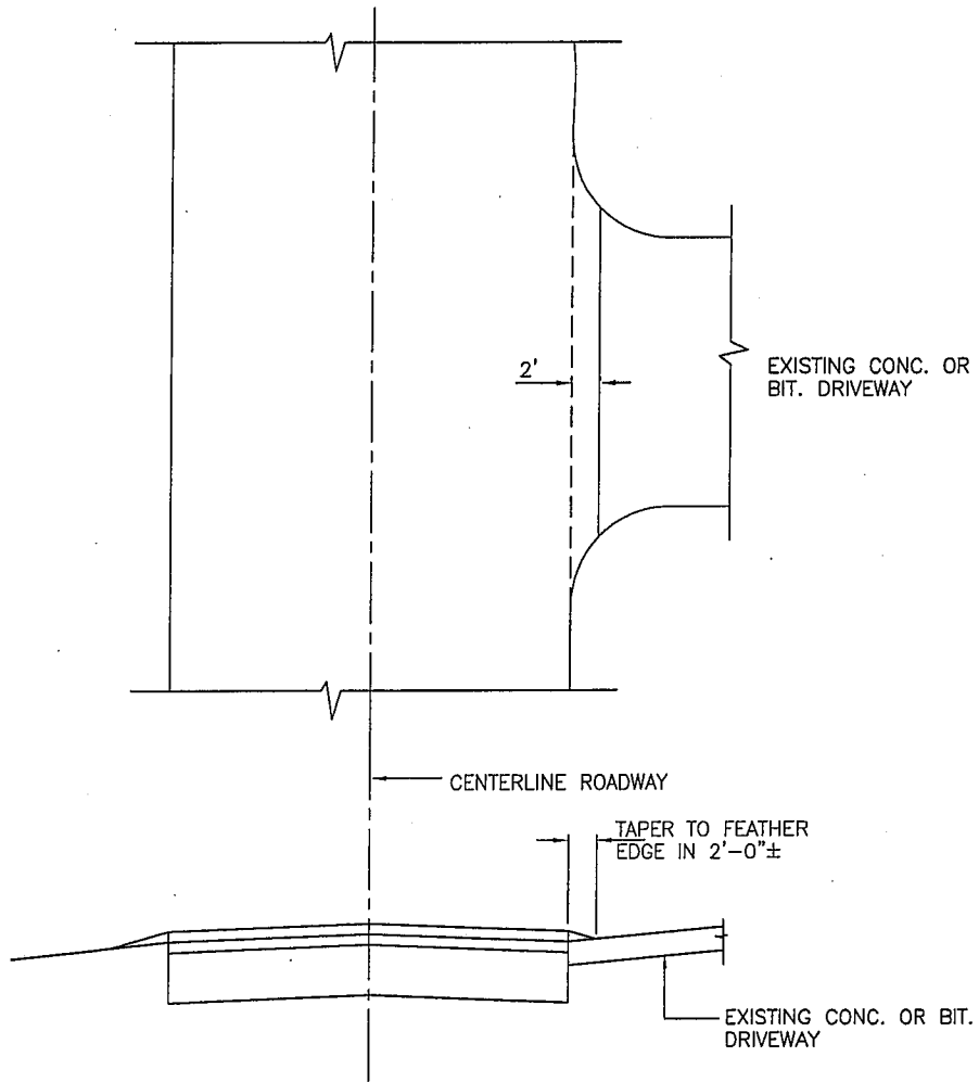
DRIVEWAY DETAIL TYPICAL
