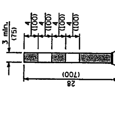
FLEXIBLE DELINEATOR
