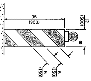
VERTICAL BARRICADE
