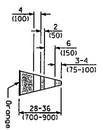
REFLECTORIZED CONE
