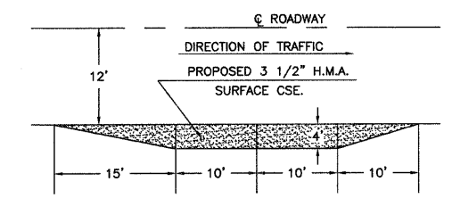
HOT-MIX ASPHALT SURFACE COURSE
