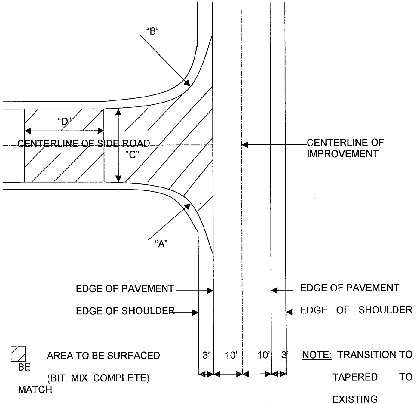
TYPICAL INTERSECTION DETAIL (SEE SCHEDULE OF INTERSECTIONS)
