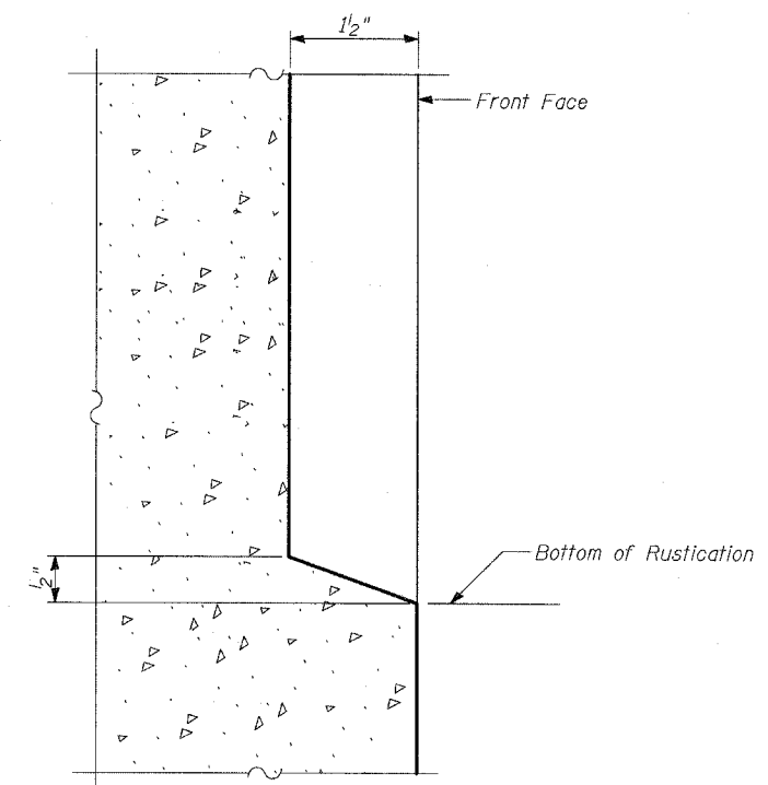
DETAIL B
