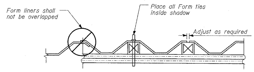
SUGGESTED FORMWORK DETAIL
