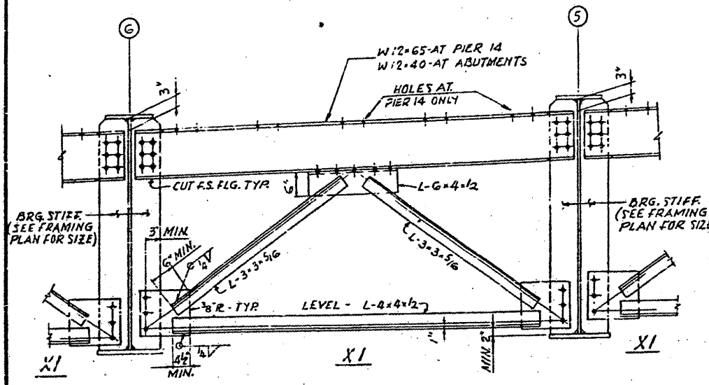
CROSSFRAME X1 (AT ABUTMENT & PIER) SCALE: 3/4" = 1'-0"
