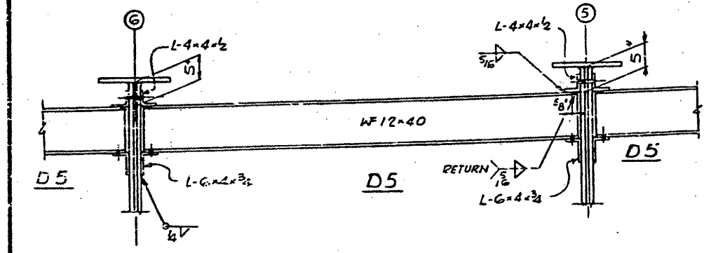
DIAPHRAGM D5 (AT LINK) SCALE: 3/4" = 1'-0"
