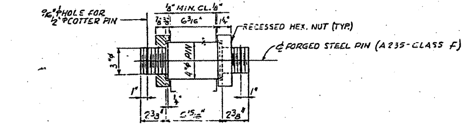
PIN DETAIL NUTS SHALL BE SHUDDERED UP FINGER TIGHT AGAINST SHOULDERS OF PIN. TOTAL NO. OF PINS REQUIRED = 14
