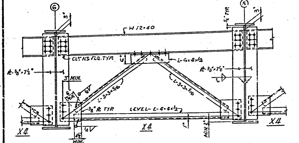
CROSSFRAME X4 (AT LINK) SCALE: 3/4" = 1'-0"
