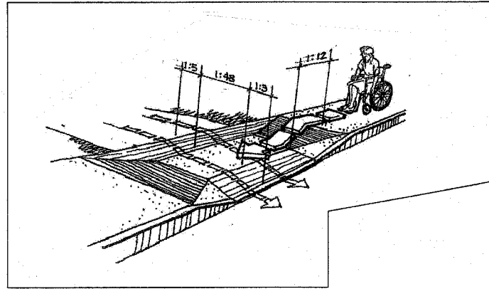
Typical Proposed Driveway Section to Meet ADA Standards
