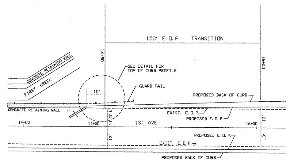
TRANSITION DETAIL OF PAVEMENT AT STA 14+50 TO STA 16+00
