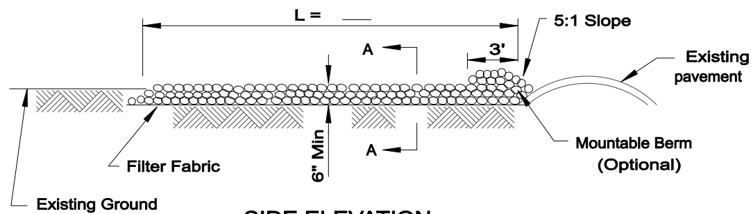
SIDE ELEVATION
