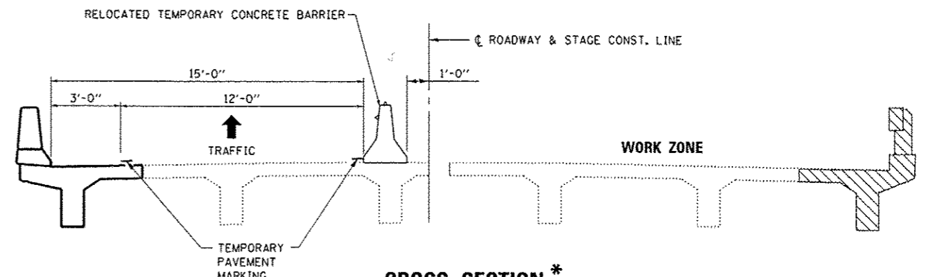
CROSS SECTION.* STAGE II STRUCTURE NO. 038-0154 (NB)
