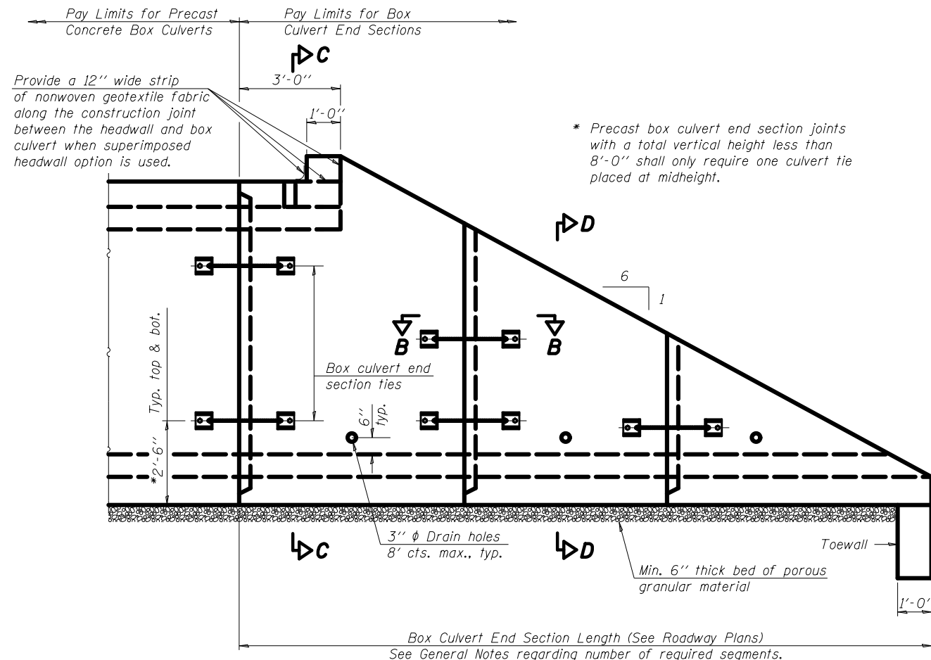
SIDE ELEVATION
