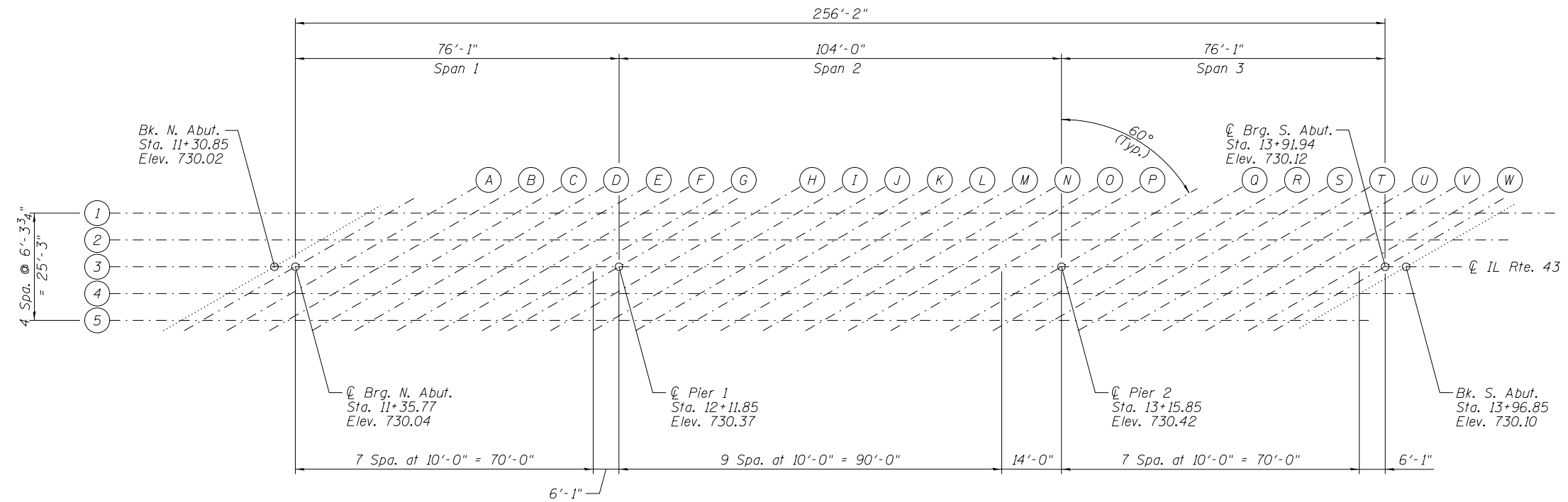
PLAN
