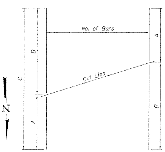
BAR CUTTING DIAGRAM
