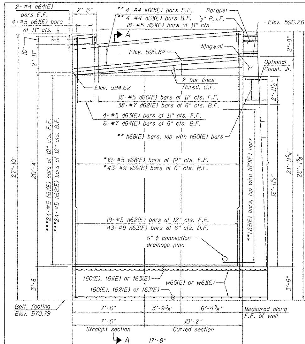
SOUTHEAST WINGWALL ELEVATION (Looking South - Drilled shafts are not shown for clarity)
