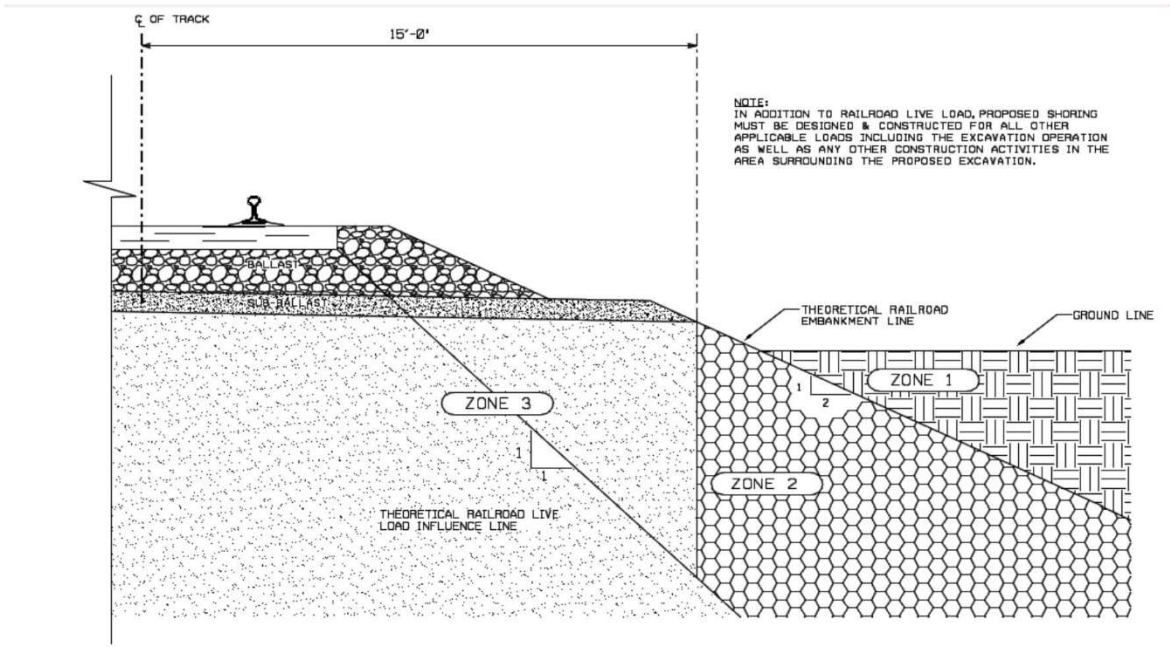
FIGURE 1: Theoretical Live Load Influence Zone
