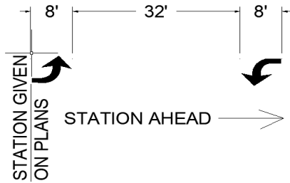
BIDIRECTIONAL TURN ARROW SPACING DETAIL
