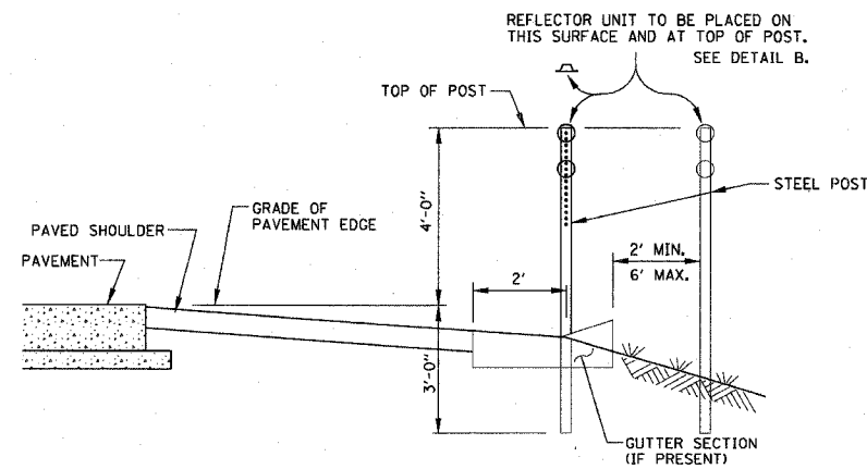
DELINEATOR INSTALLATION
