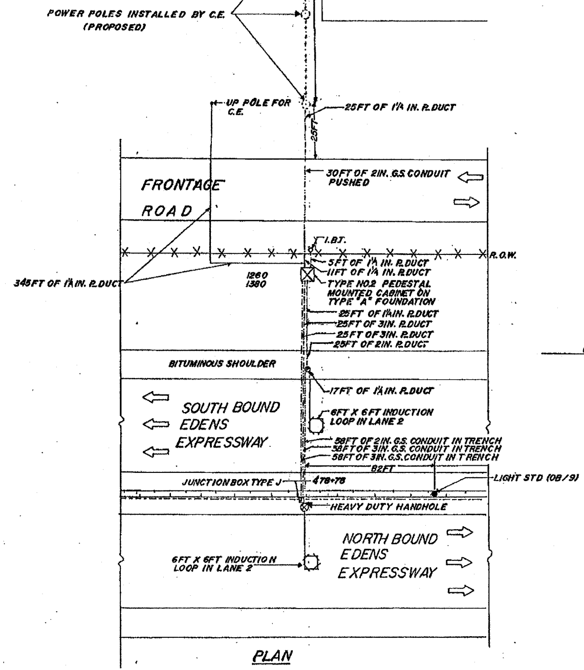
WIRING DIAGRAM
