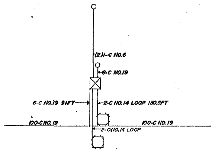
WIRING DIAGRAM
