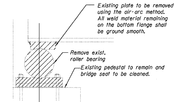
EXISTING ABUT. ELEVATION AT BEAMS 1 AND 5 THRU 20
