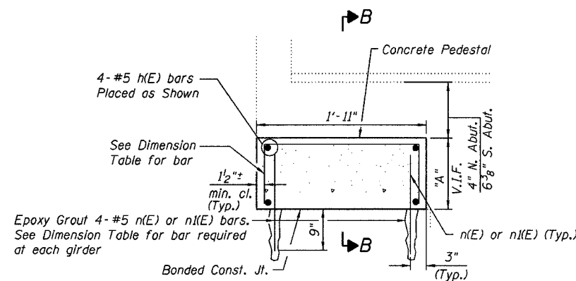
PROPOSED ABUT. ELEVATION AT BEAMS 1, 5 THRU 11 AND 20 (Brg. omitted for clarity)
