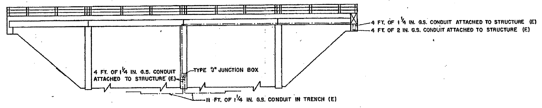
NORTH ELEVATION
