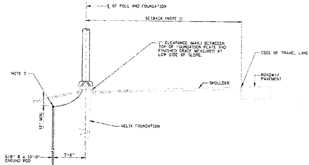
TYPICAL INSTALLATION OUTSIDE CLEAR ZONE NO SCALE
