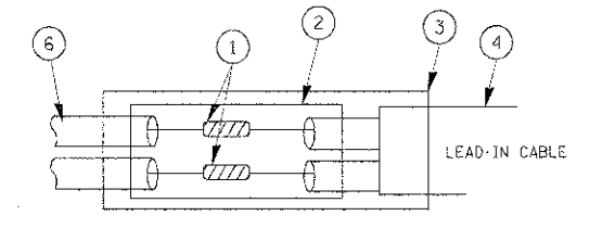
DETAIL "B" LOOP-TO-CONTROLLER SPLICE
