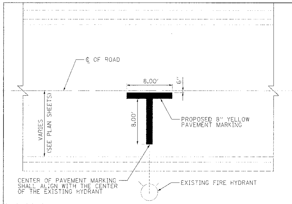
HYDRANT TEE PAVEMENT MARKING DETAIL N.T.S.
