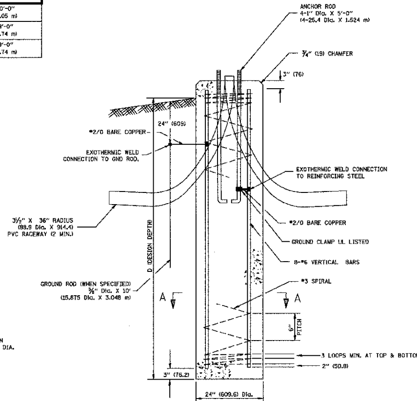
FOUNDATION DETAIL
