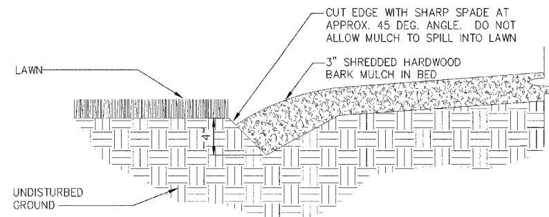
SPADE EDGING DETAIL
