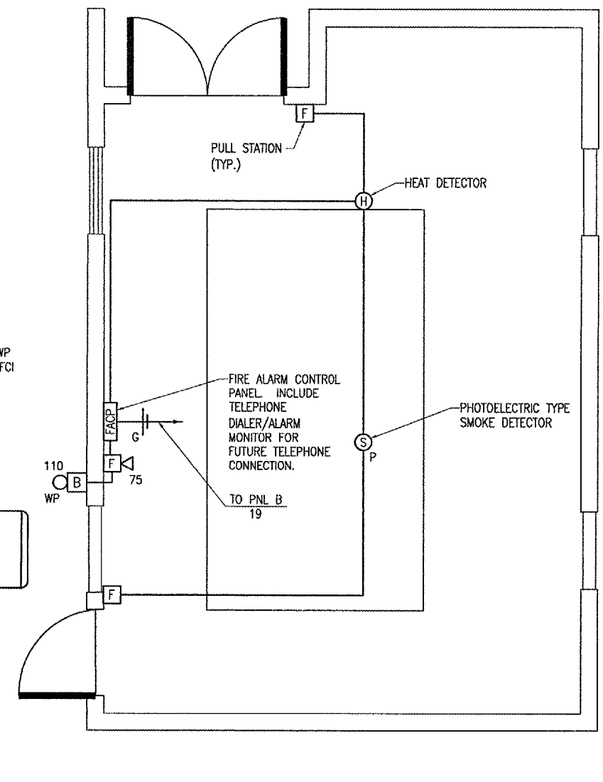
FIRE ALARM DETECTION PLAN SCALE 3/8"=1'-0" 2 0 2 4 FEET
