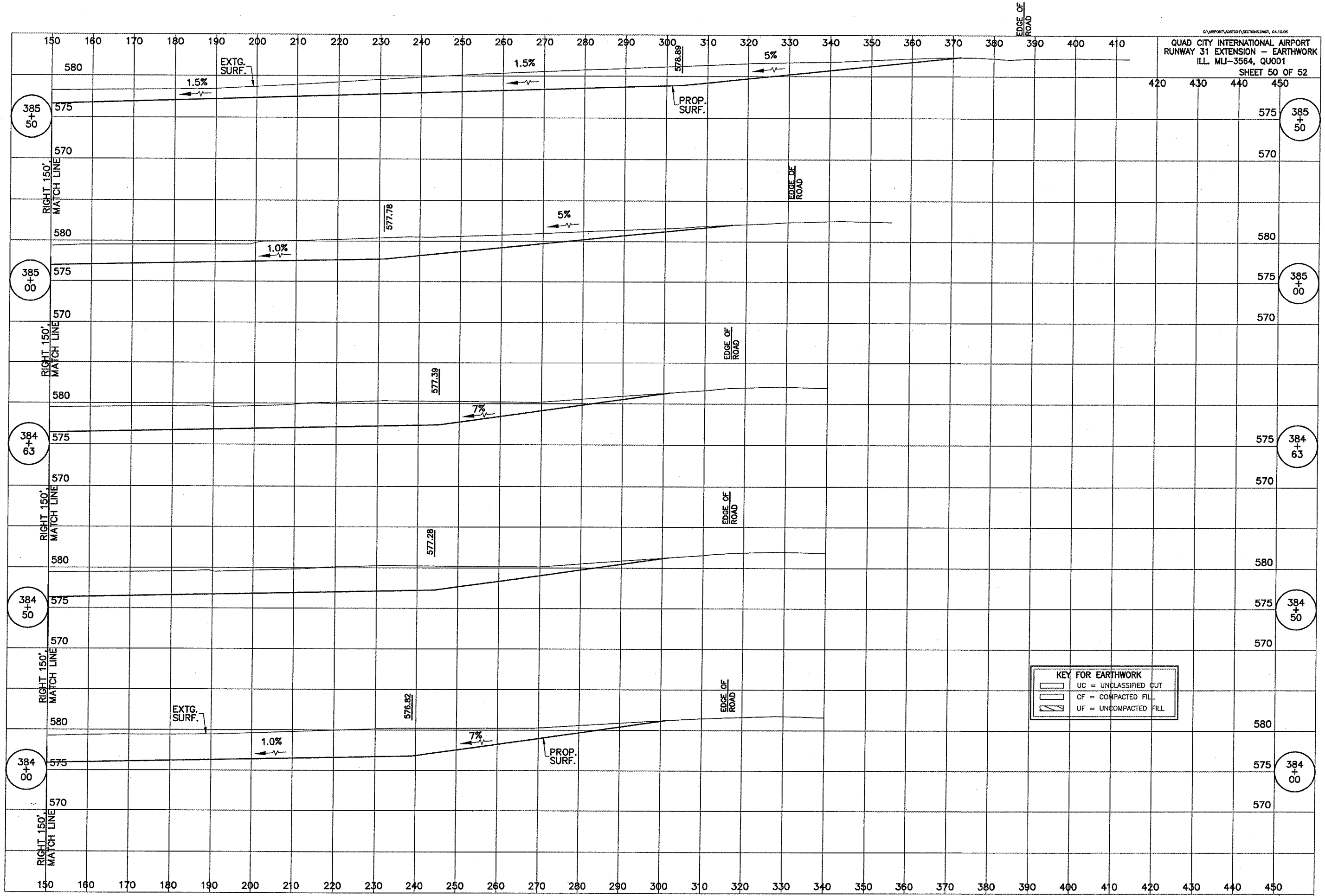
TAXIWAY K RIGHT CROSS SECTIONS, STA 384+00 TO STA 385+50
