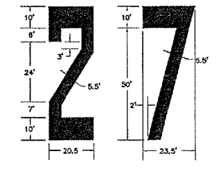
PROPOSED NUMERAL DETAILS "NOT TO SCALE"
