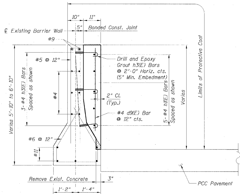
DETAIL 3
