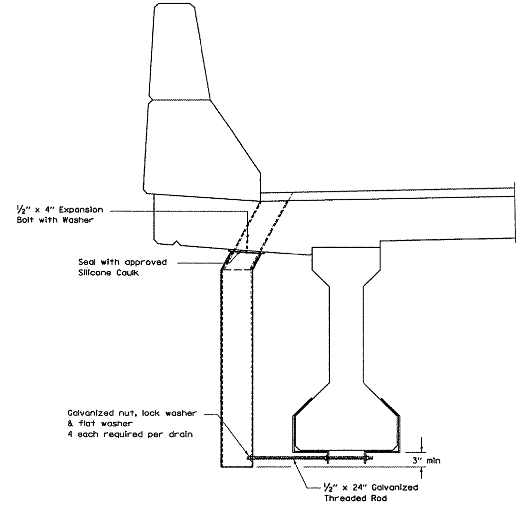
SECTION AT PARAPET
