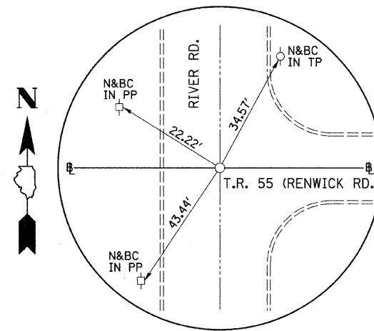
SECTION CORNER STA. 126+93.50 T.R. 55 (RENWICK RD.) N. 9969.717, E. 7730.190 (MAG NAIL)
