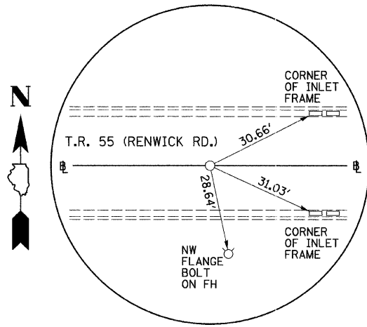
P.O.T. STA. 105+00.00 T.R. 55 (RENWICK RD.) N. 9987.722, E. 5536.764 (MAG NAIL)
