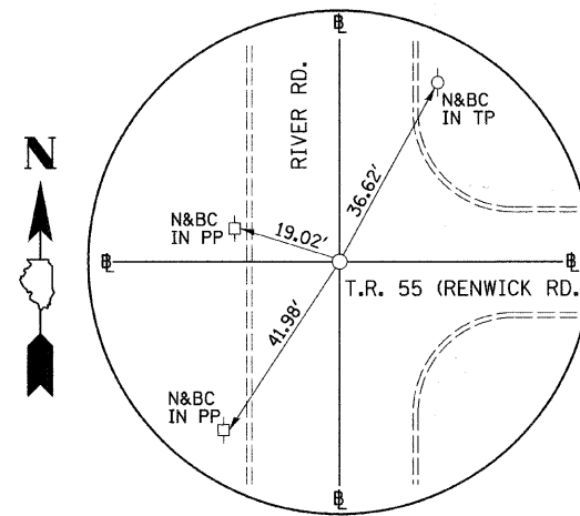
P.O.T. STA. 126+90.28 T.R. 55 (RENWICK RD.) = P.O.T. 13+46.10 (RIVER RD.) N. 9969.696, E. 7726.970 (MAG NAIL)
