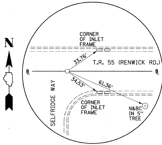
P.O.T. STA. 100+50.00 T.R. 55 (RENWICK RD.) N. 9991.425, E. 5086.779 (MAG NAIL)
