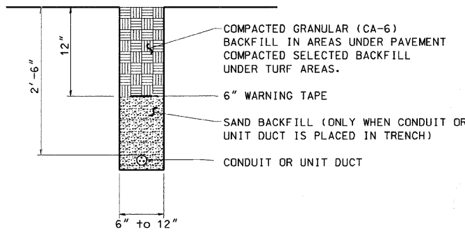
TRENCH AND BACKFILL
