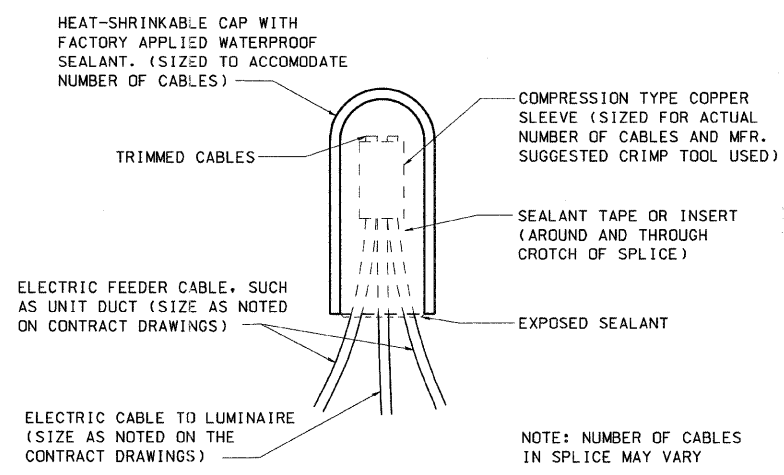
SPLICING ELECTRIC CABLE
