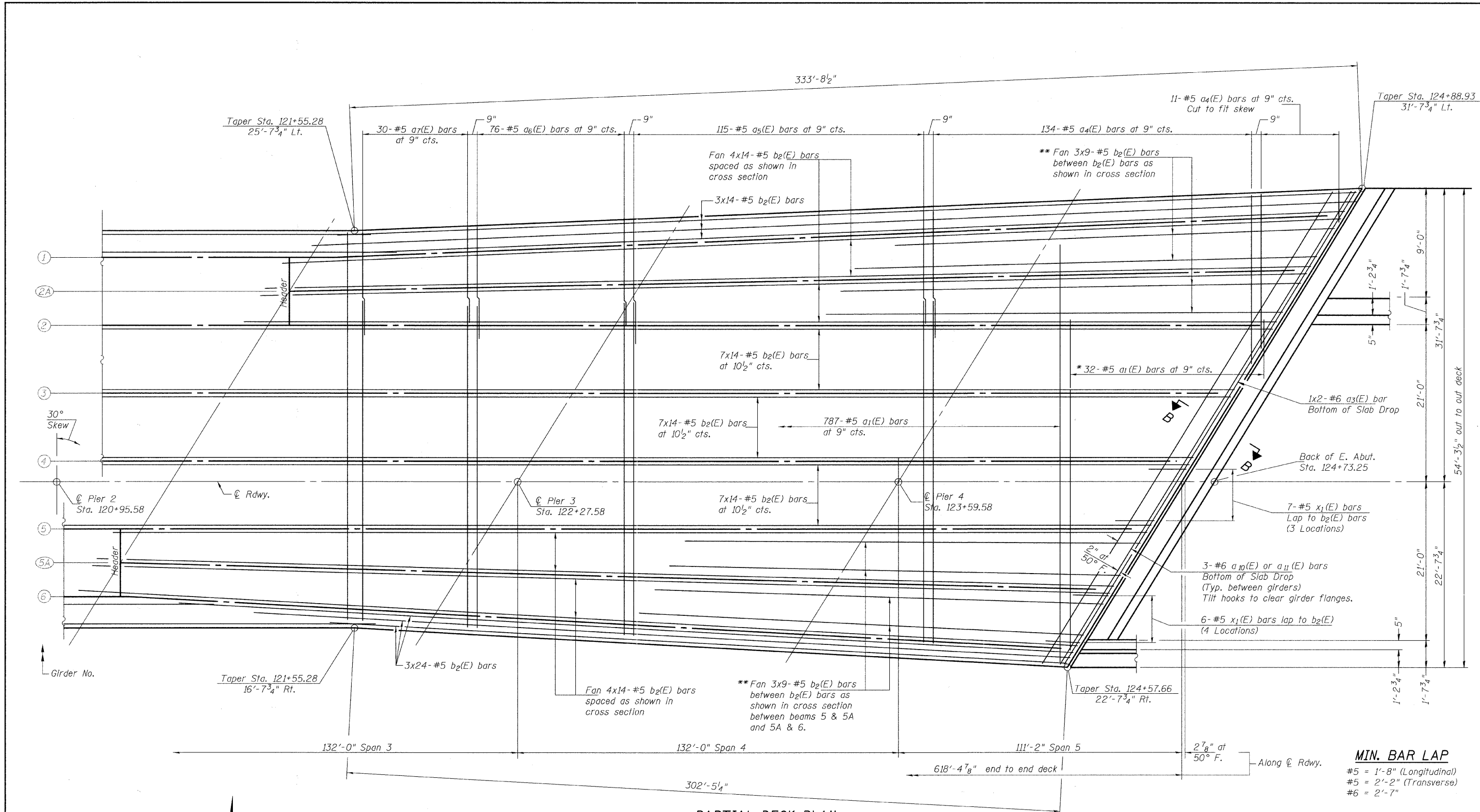
PARTIAL DECK PLAN (Showing Bottom Reinforcement Bars in Spans 3, 4 & 5)
