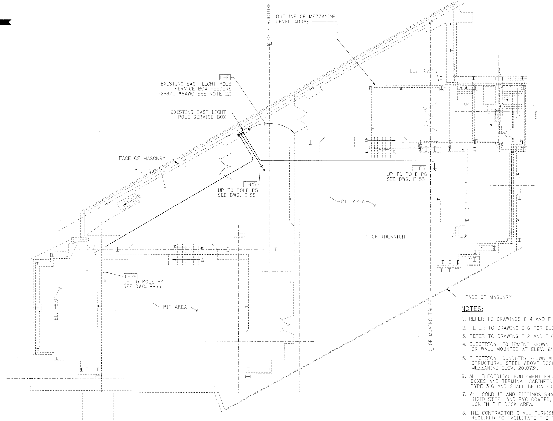
PLAN 1/8"=1'-0"
