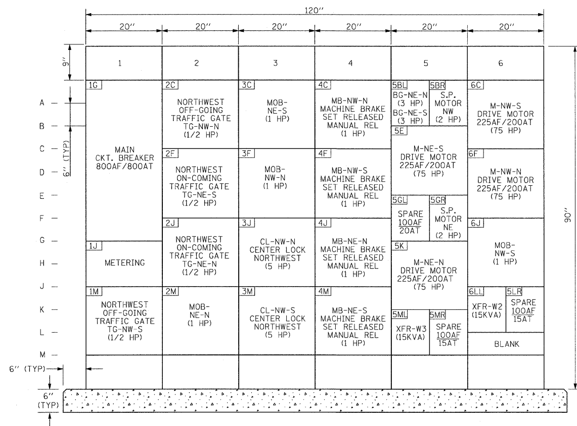
WESTBOUND MCC-WB-1 FRONT ELEVATION
