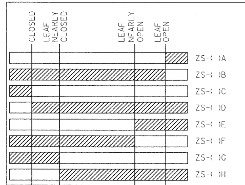
ROTARY LIMIT SWITCHES ZS-NE, ZS-NW, ZS-SE & ZS-SW
