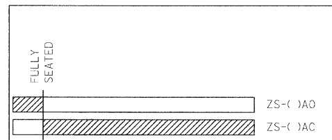
FULLY SEATED LIMIT SWITCHES ZS-NEFS, ZS-NWFS, ZS-SEFS & ZS-SWFS
