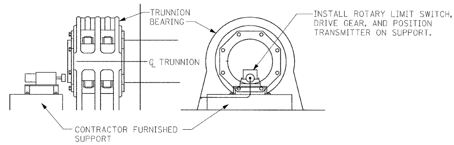
DETAIL ROTARY LIMIT SWITCH AND POSITION TRANSMITTER N.T.S.
