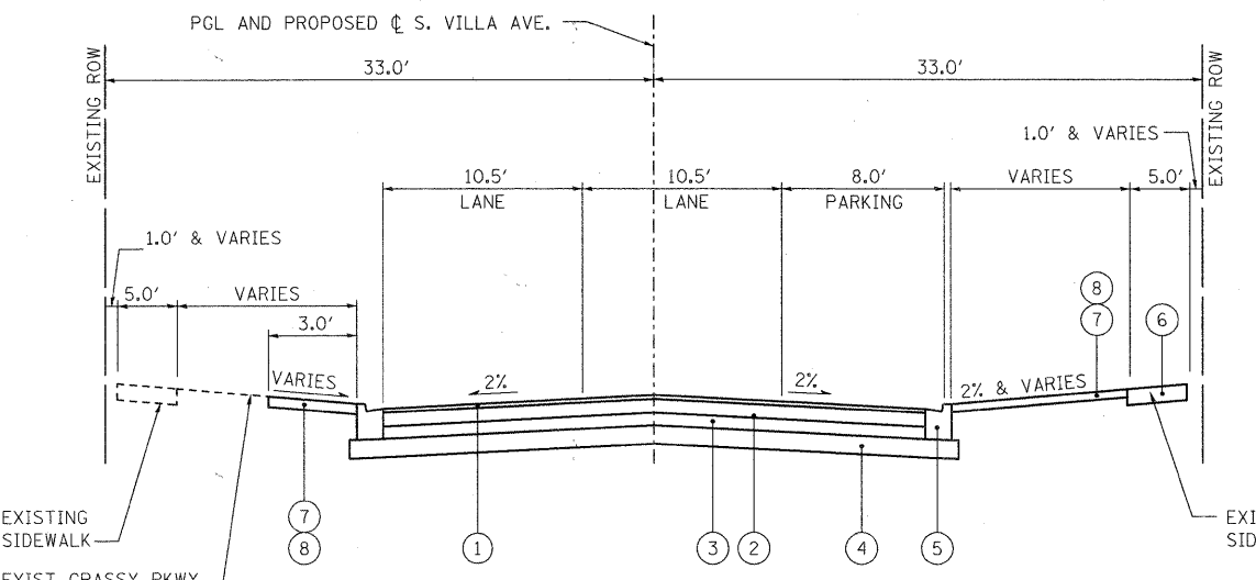
PROPOSED TYPICAL SECTION 250' NORTH OF MADISON STREET TO CRESCENT DR STA 66+16 TO 98+41.50
