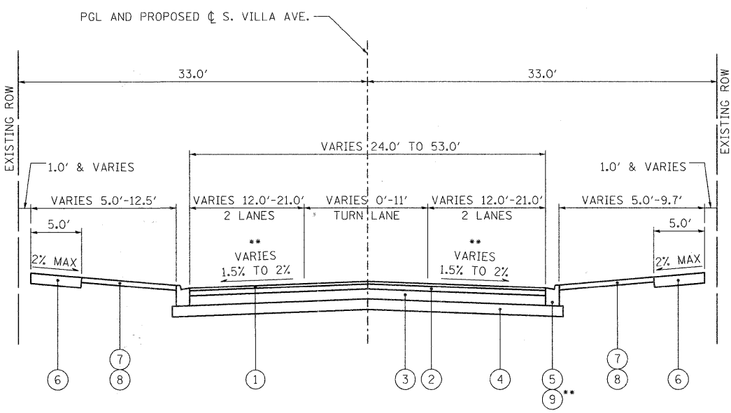
PROPOSED TYPICAL SECTION 105' NORTH OF WILDWOOD AVENUE TO ST. CHARLES ROAD STA 110+52 TO 116+71.35
