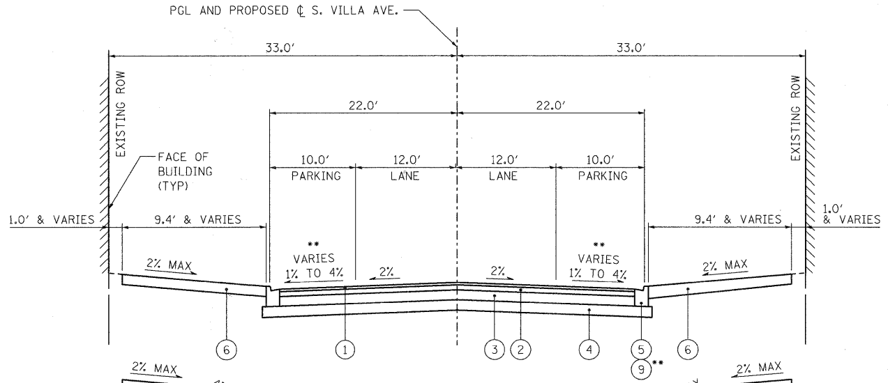
PROPOSED TYPICAL SECTION CENTRAL BOULEVARD TO 105' NORTH OF WILDWOOD AVENUE STA 102+50 TO 110+52
