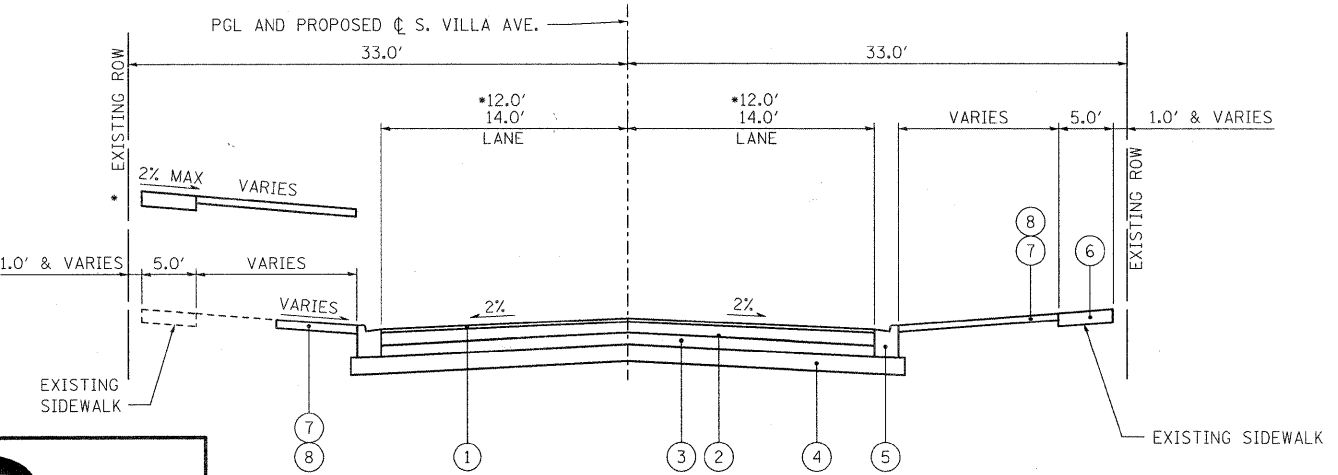
PROPOSED TYPICAL SECTION CRESCENT DR. TO E. PARK BLVD. STA 98+41.50 TO STA 102+50
