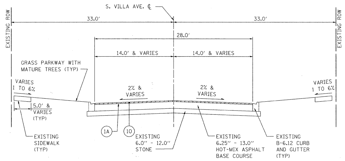
PROPOSED TYPICAL SECTION STA 63+19.78 TO STA 66+16.00
