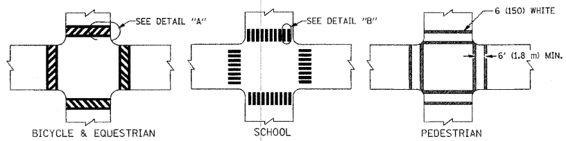
BICYCLE & EQUESTRIAN
