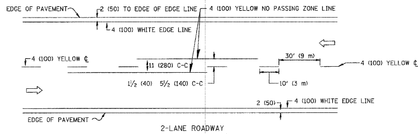
2-LANE ROADWAY
