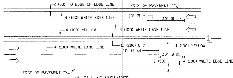
MULTI-LANE UNDIVIDED
