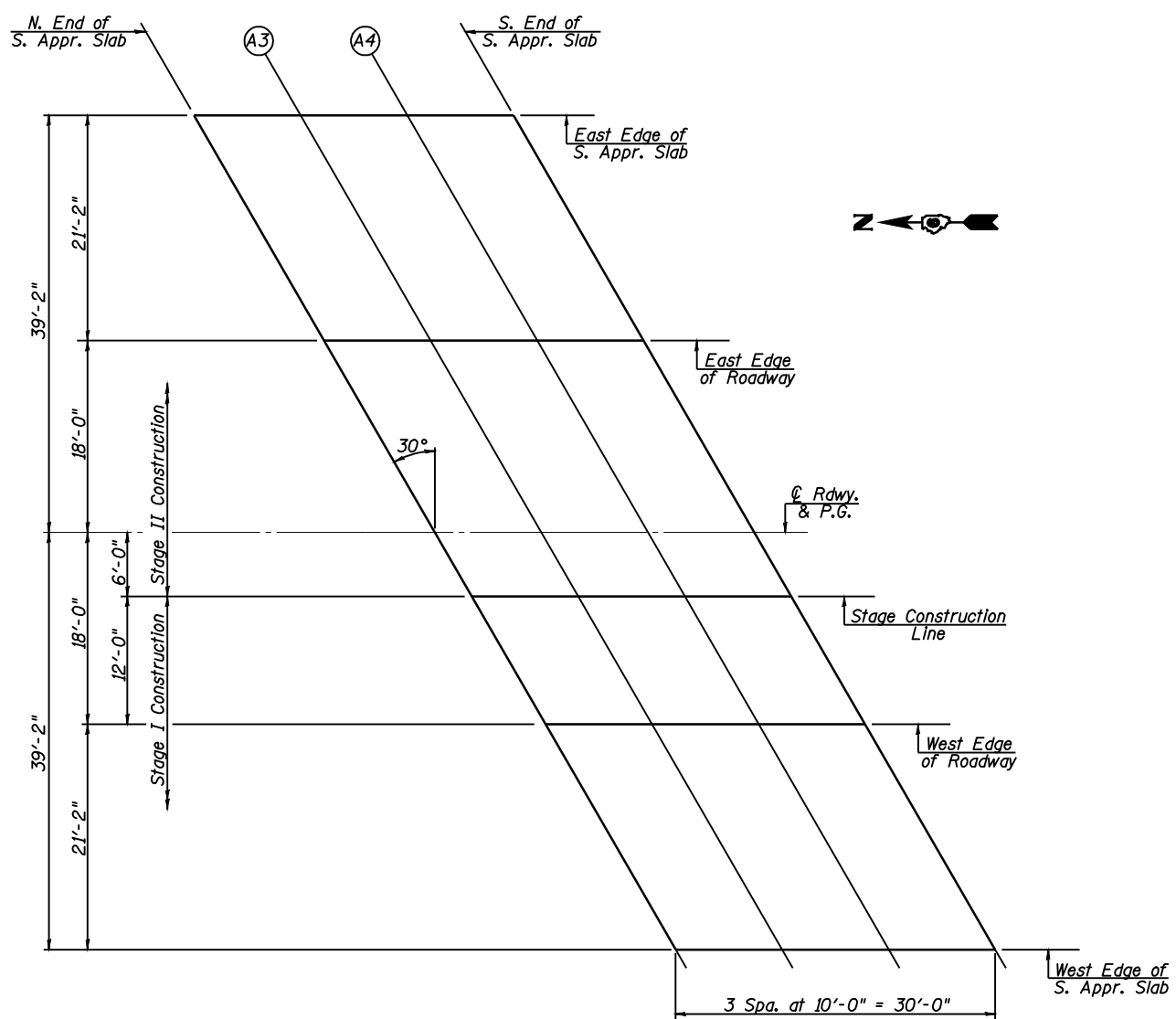
LAYOUT PLAN - S. APPROACH ELEVATIONS
