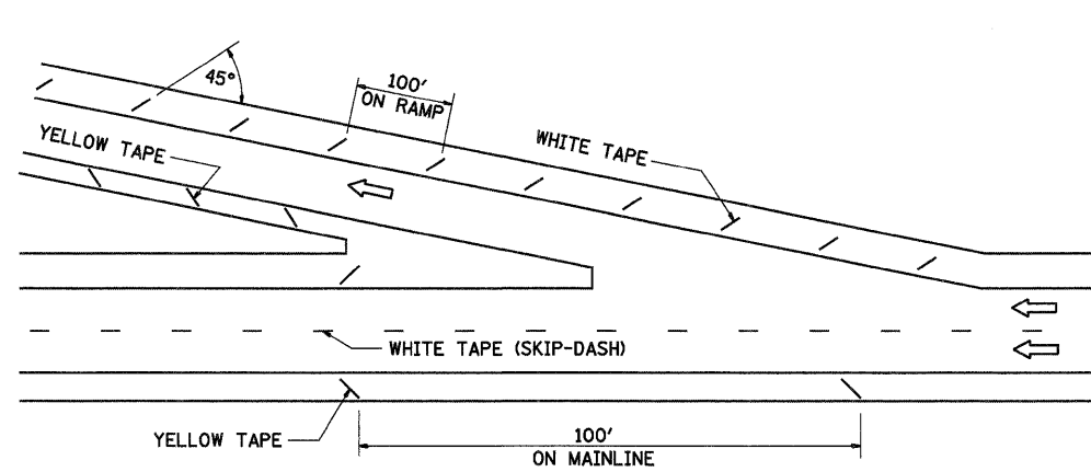
TYPICAL EXIT TERMINAL
