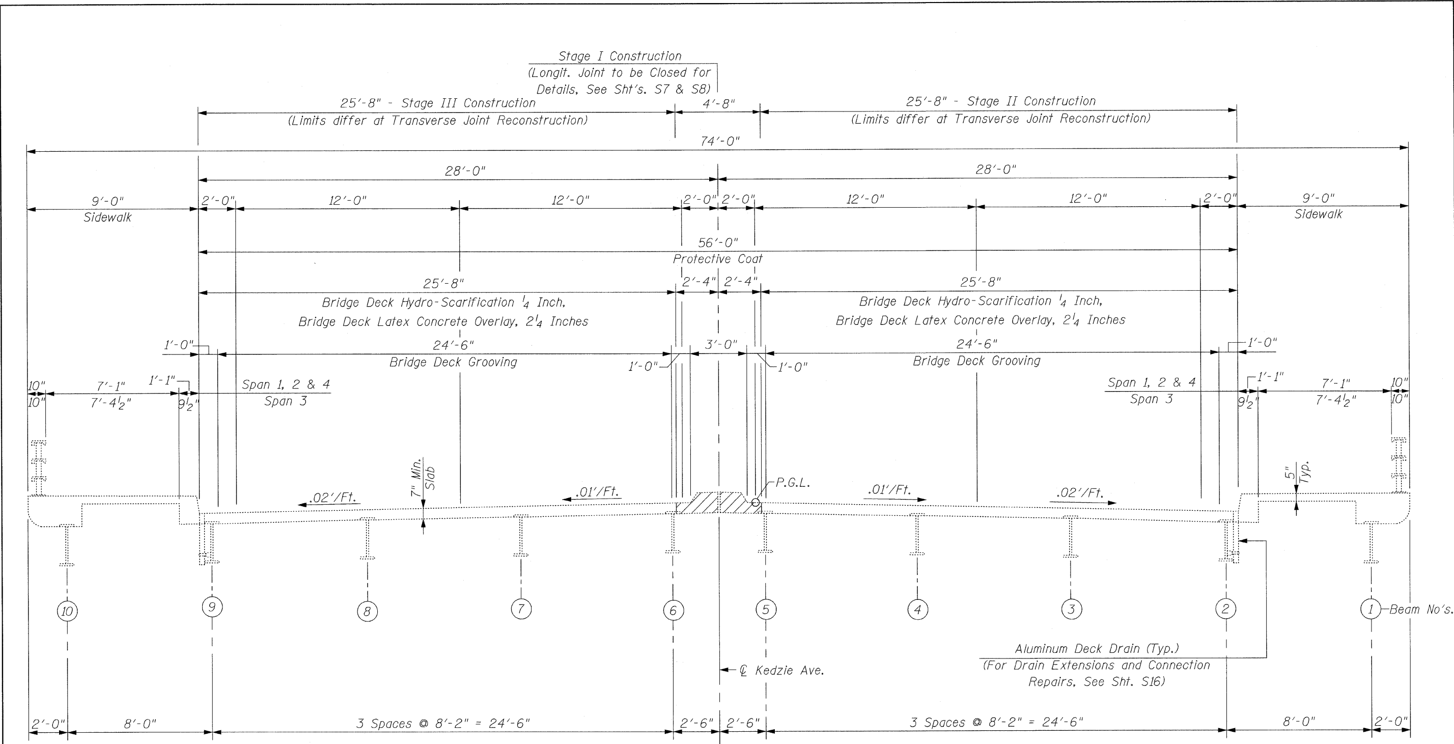
EXISTING DECK CROSS SECTION (Looking North)
