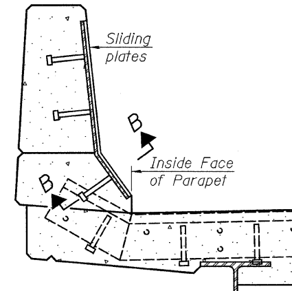
SECTION A-A POINT BLOCK DETAILS (for skews > 30°)
