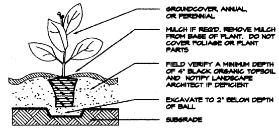
6 PERENNIAL L1.0 NOT TO SCALE
