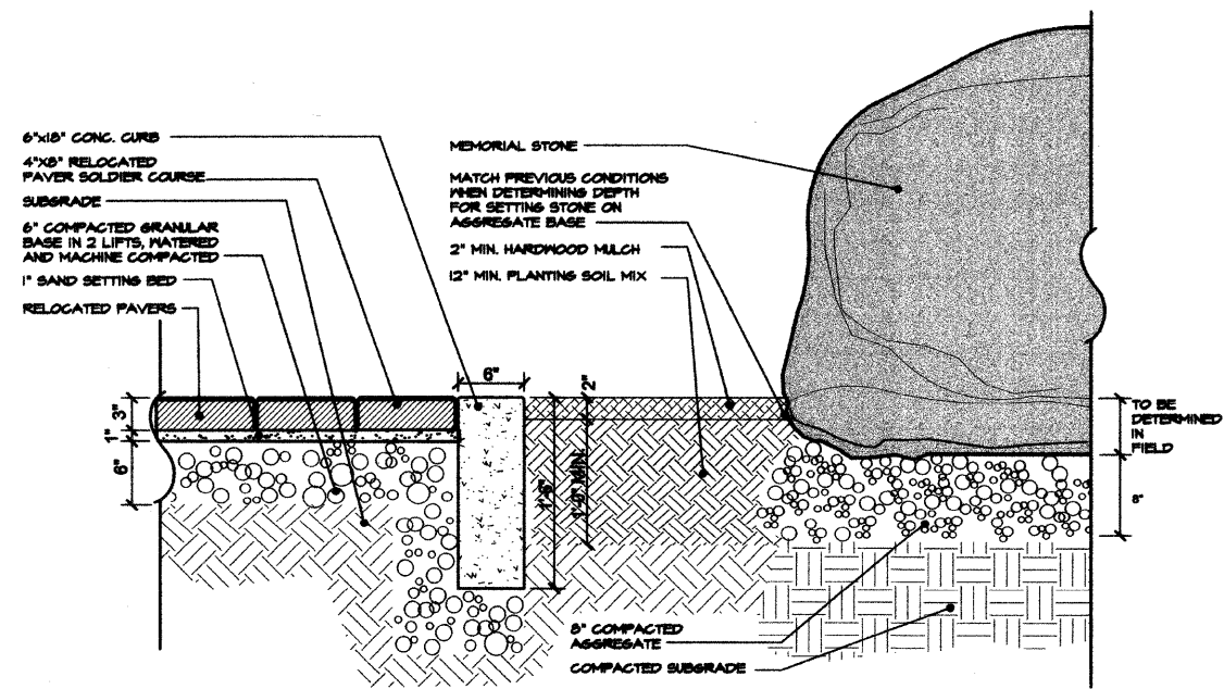
2 MEMORIAL STONE PLANTING BED AND PAVERS L1.0 SCALE: 1/8" = 1'-0"
