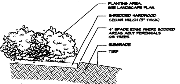
5 NATURAL SPADE EDGE L1.0 NOT TO SCALE
