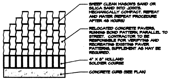
4 RELOCATED PAVERS L1.0 NOT TO SCALE
