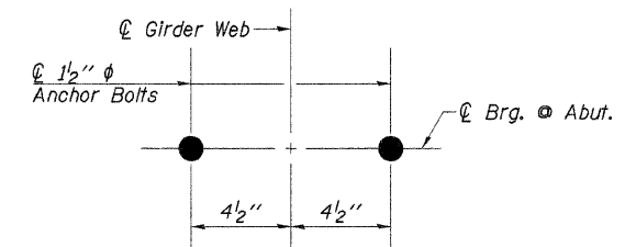
ANCHOR BOLT LOCATION PLAN
