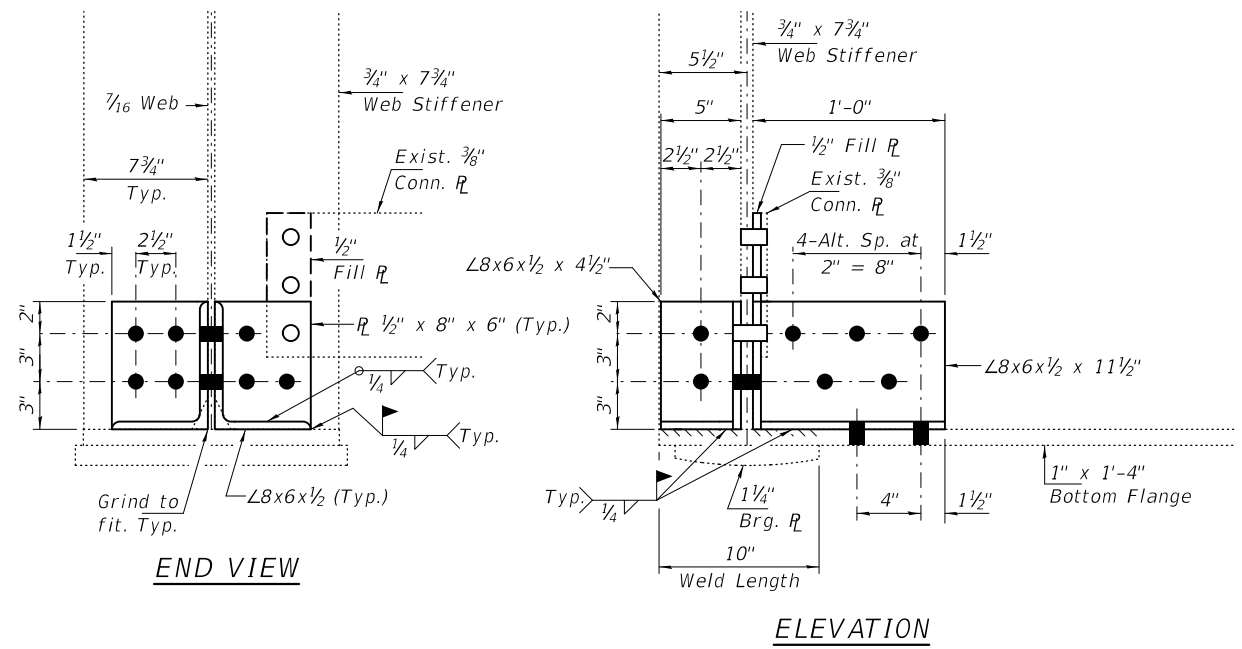
GIRDER REPAIR "A" (4-Locations)
