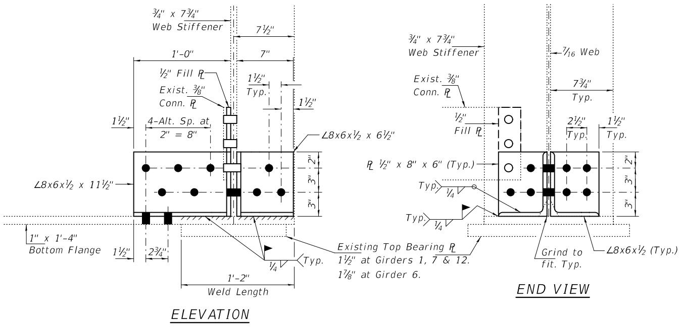
GIRDER REPAIR "B" (4-Locations)
