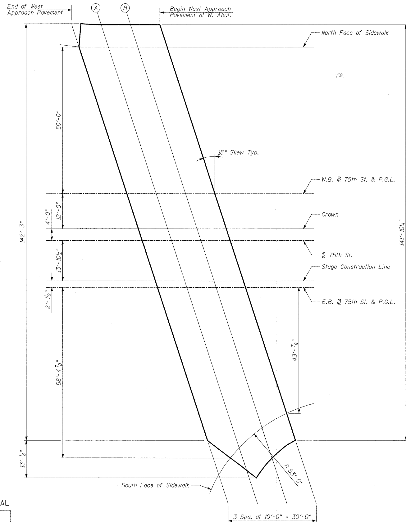
PLAN
