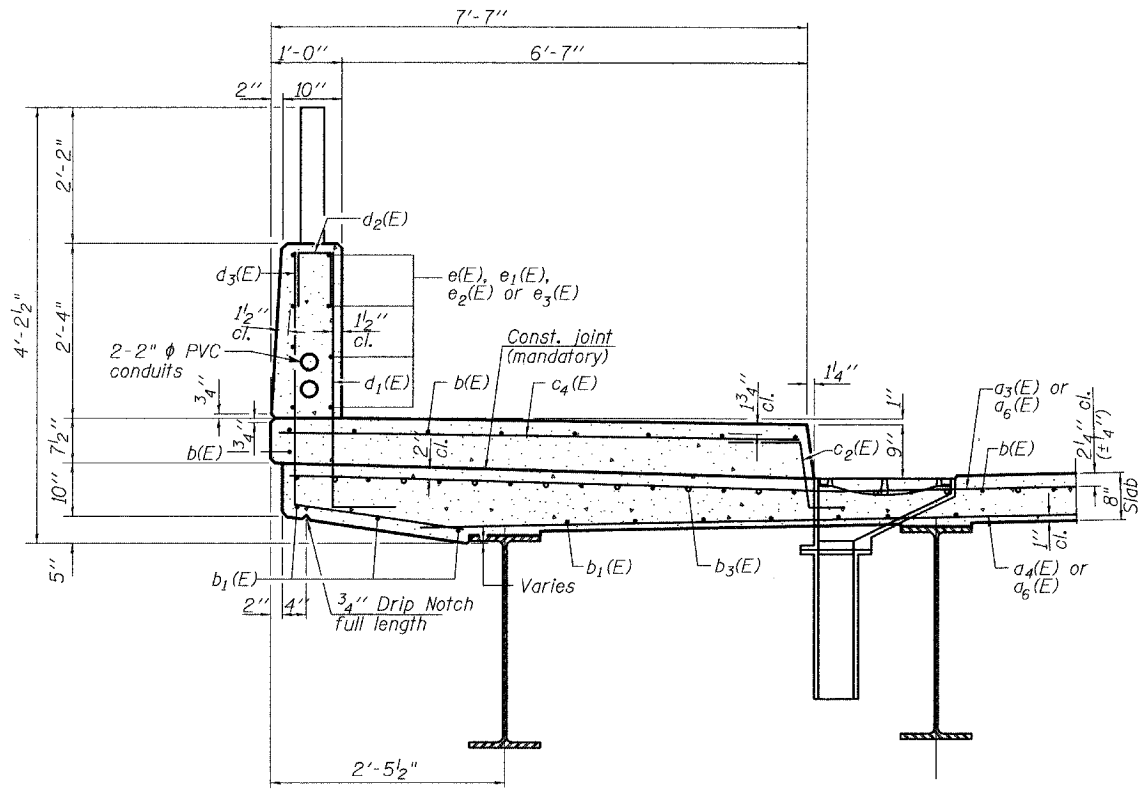
SECTION THRU NORTH SIDEWALK
