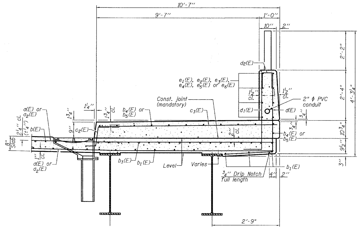
SECTION THRU SOUTH SIDEWALK
