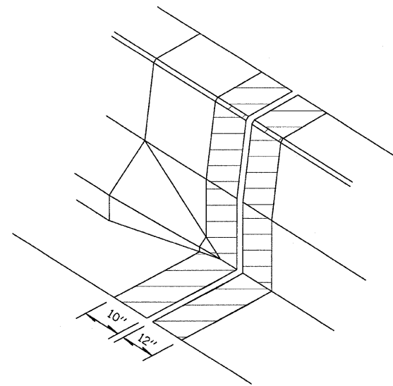
TYPICAL CONCRETE REMOVAL AT WEST ABUTMENT
