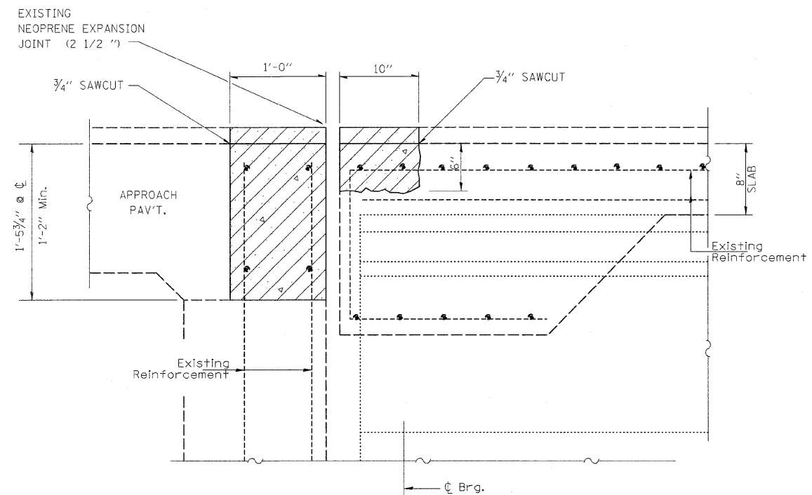
EXISTING EXPANSION JOINTS AT ABUTMENT
