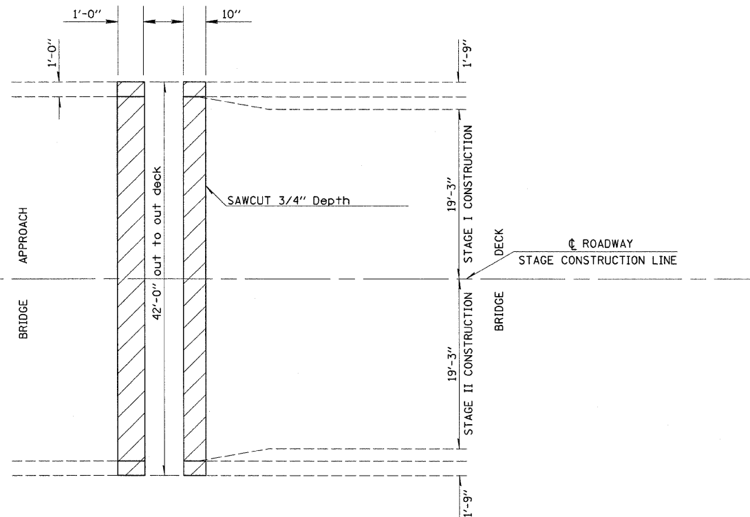
REMOVAL PLAN VIEW WEST ABUTMENT
