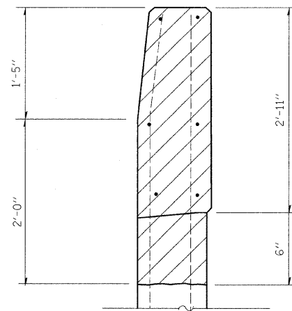
WINGWALL DETAIL
