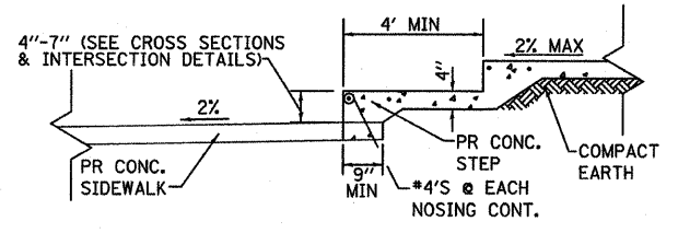
TYPICAL STEP DETAIL "B" (STA. 22+90.14) (FOR STAIR CASES WITH 1 STEP OR RISERS 4' OR MORE APART)
