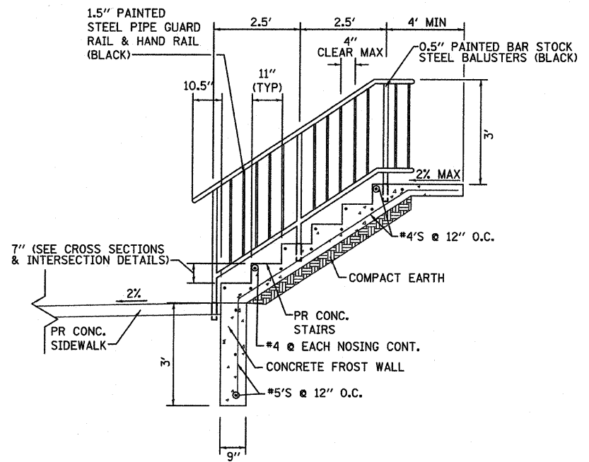
TYPICAL STAIR CASE DETAIL "A" (FOR STAIR CASES WITH 2 OR MORE STEPS)
